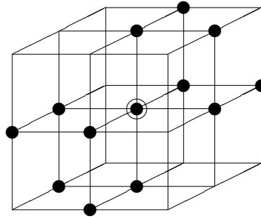
Figure 2: Finite difference stencil for 3D explicit time-marching
