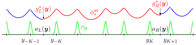
FIGURE 5.1. An illustration of the first a/c method. In \Omega^{\text{at}} = (a_L(\mathbf{y}), a_R(\mathbf{y})) the atomistic problem is solved with the Dirichlet boundary conditions g^*(\mathbf{y}) . Outside \Omega^{\text{at}} the Cauchy–Born approximation is used in all cells Q_j .
