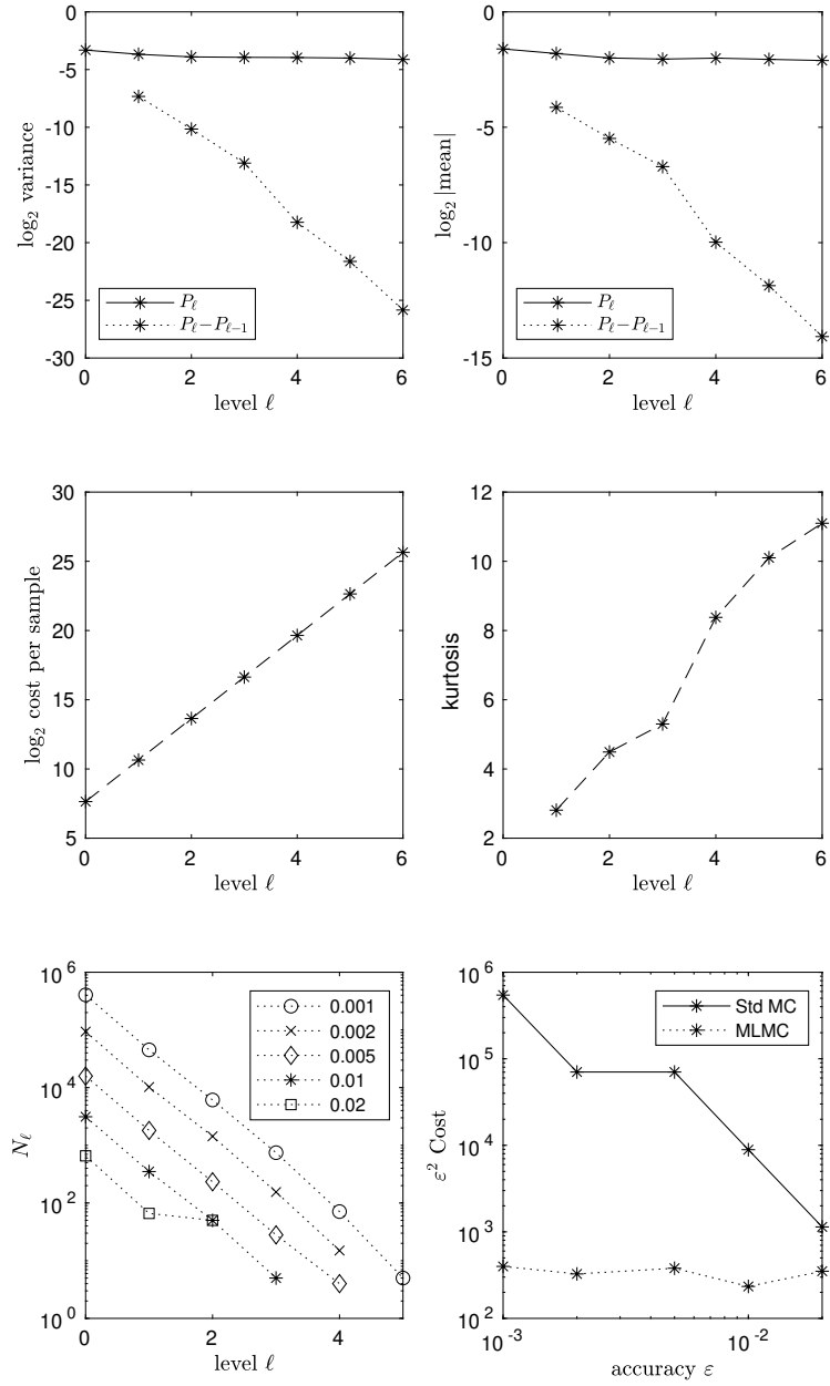
Figure 1: Zakai SPDE arising from modelling credit derivatives
