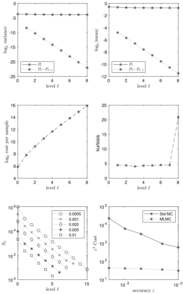
Figure 2: MLMC using projection at boundary
