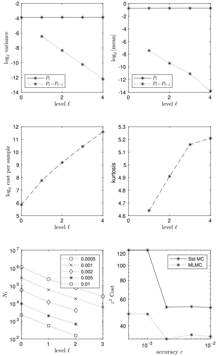
Figure 1: MLMC using reflection scheme at boundary
