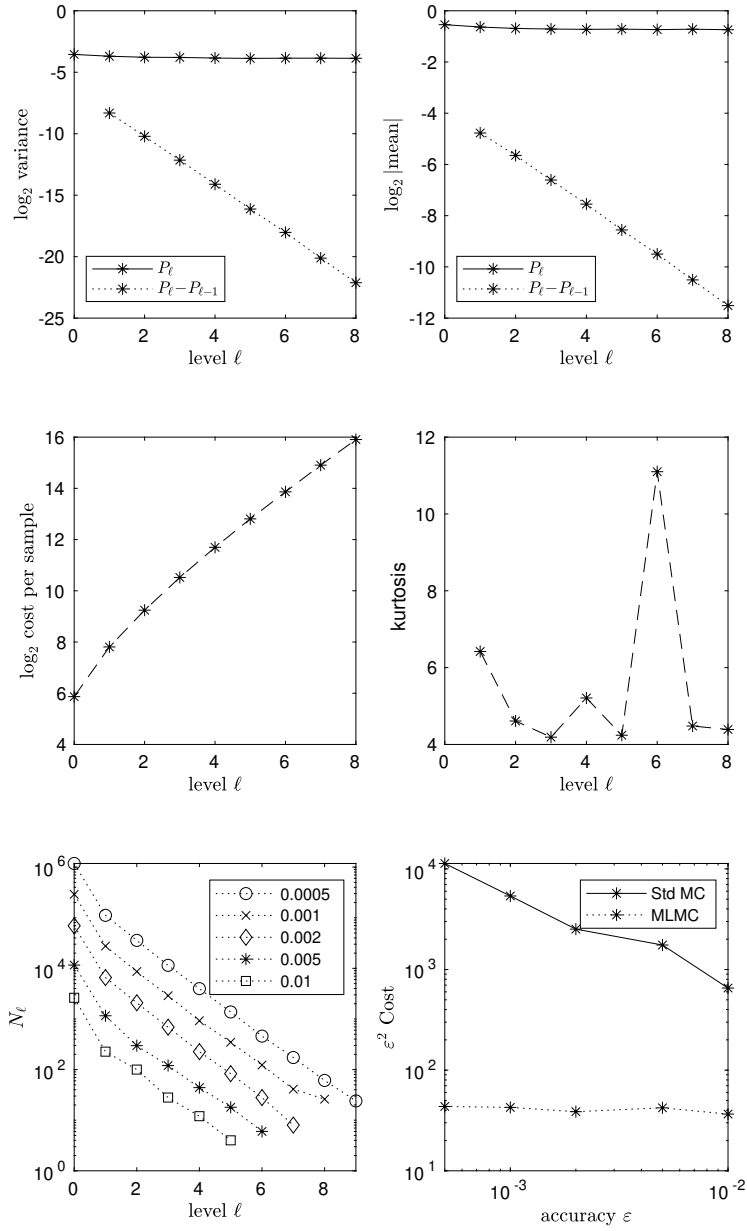
Figure 3: MLMC using penalisation at boundary
