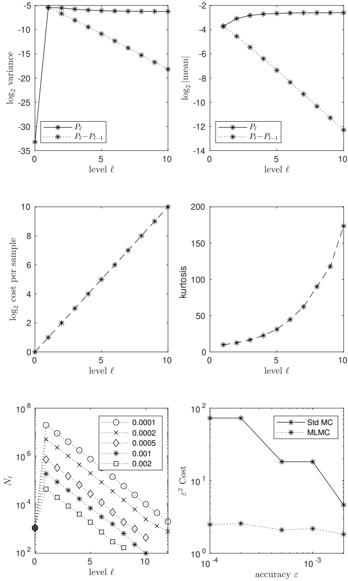
Figure 1: Simple nested expectation estimation of EVPPI
