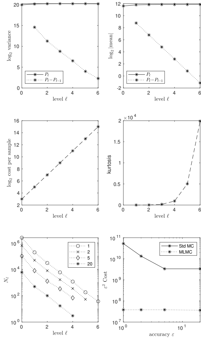
Figure 1: MLMC results for continuous time Markov process
