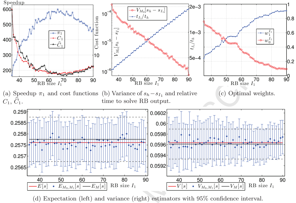
Figure 3: Result for the 1-MVR method vs RB size I_1 .
