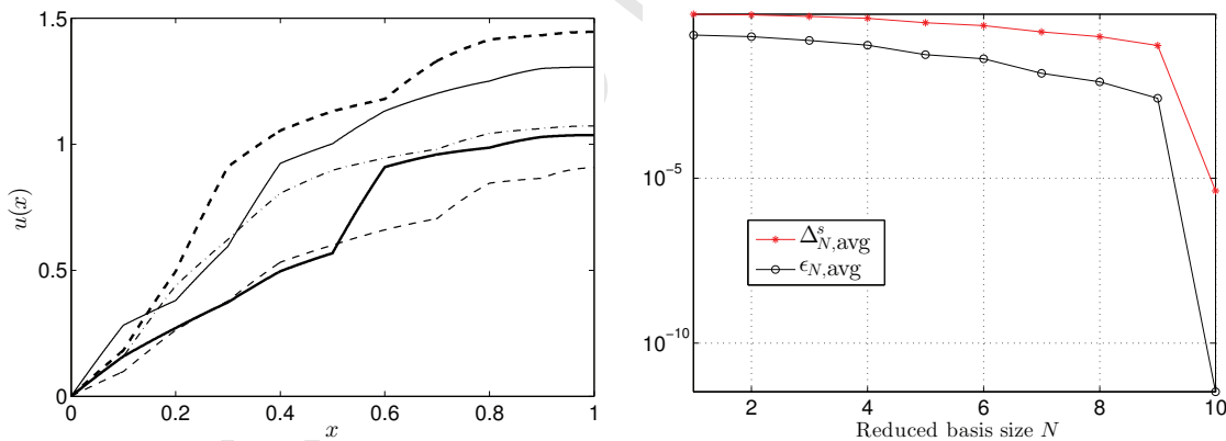
(a) Exact solution u(x, \mathbf{y}) for several realizations of the diffusivity field. (b) Average output error bound \Delta_{N, \text{avg}}^s and average output error \epsilon_{N, \text{avg}} for \mathbf{y} \in Y_{\widehat{M}} vs. RB size N .
