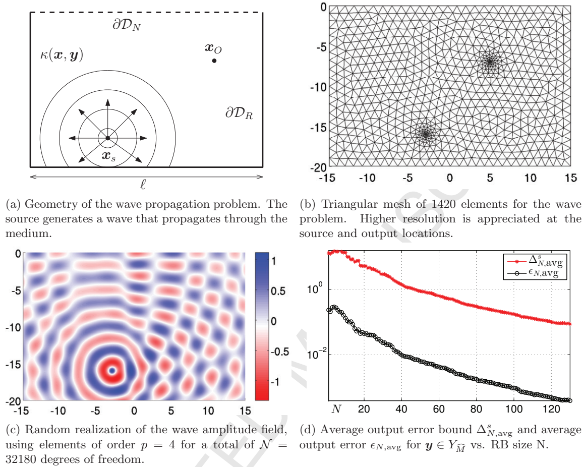
Figure 2: Problem specification, representative solution, and RB convergence of the wave propagation example
